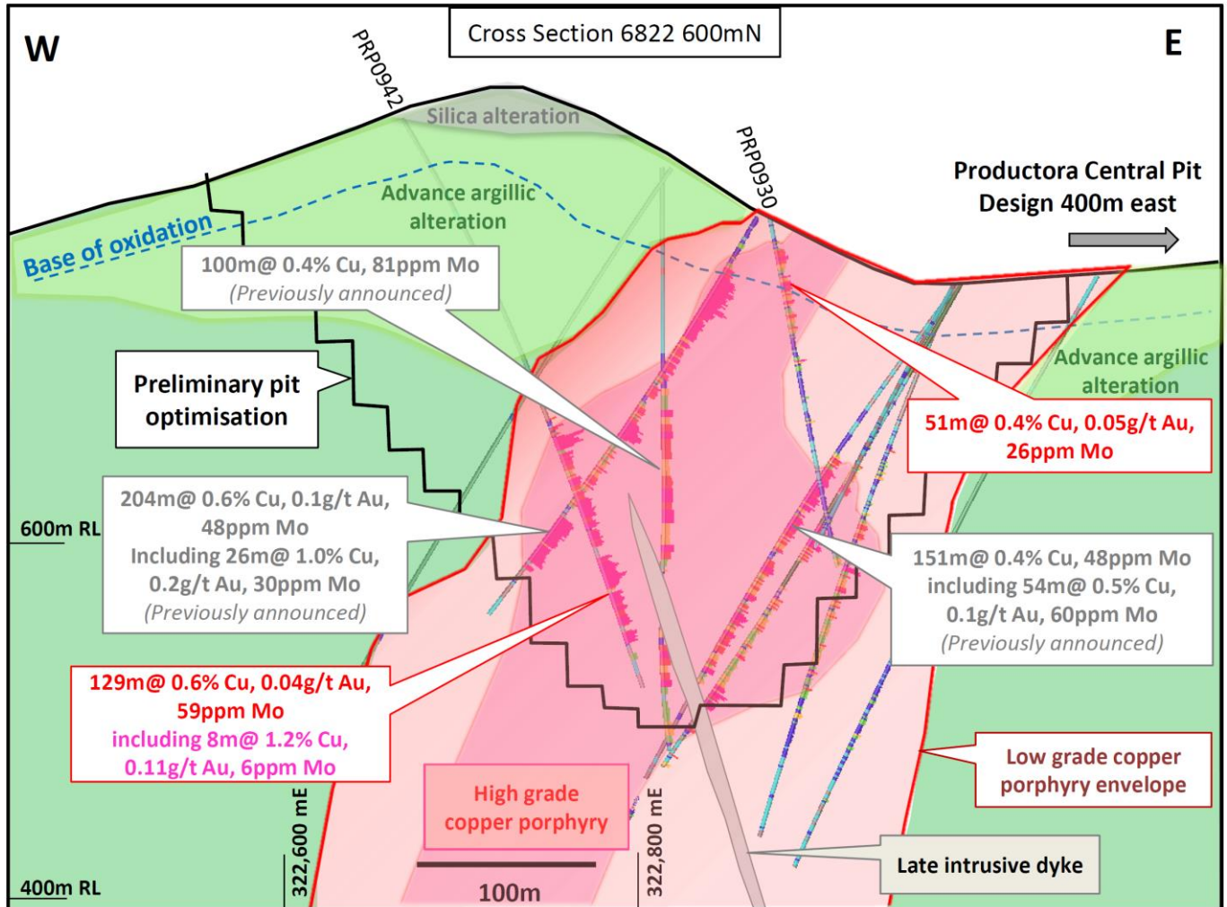
Figure 2. Cross section displaying the location of new copper drilling intersections at the Alice copper porphyry deposit, Productora copper project.
