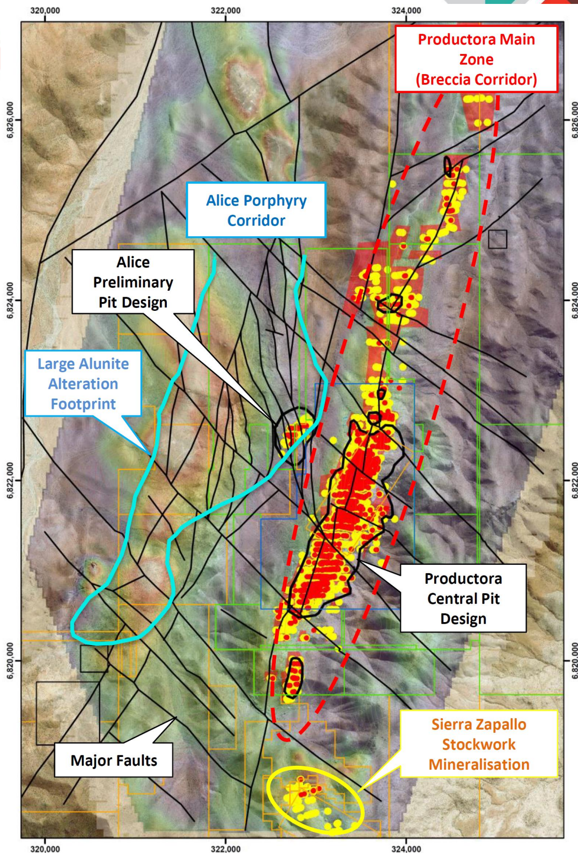
Figure 1. Plan displaying the location of the Alice copper porphyry discovery in relation to the planned Productora central pit design, Mineral Resource outlines and TMI.
